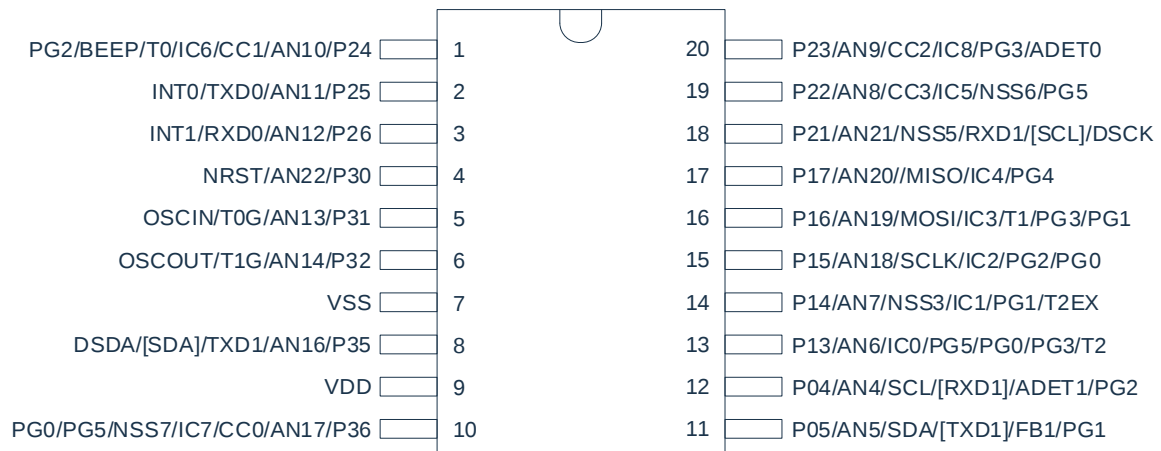
CMS8S5880-TSSOP20
