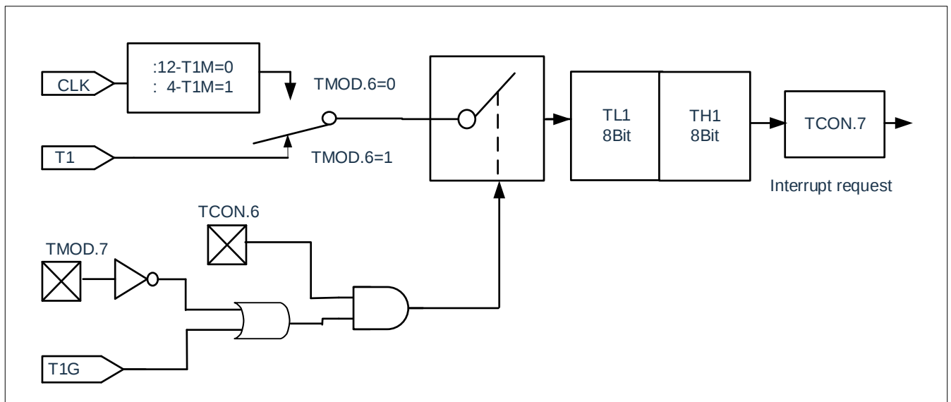
Figure 8-6: Timer1, Mode 1: 16-bit timing/counter
