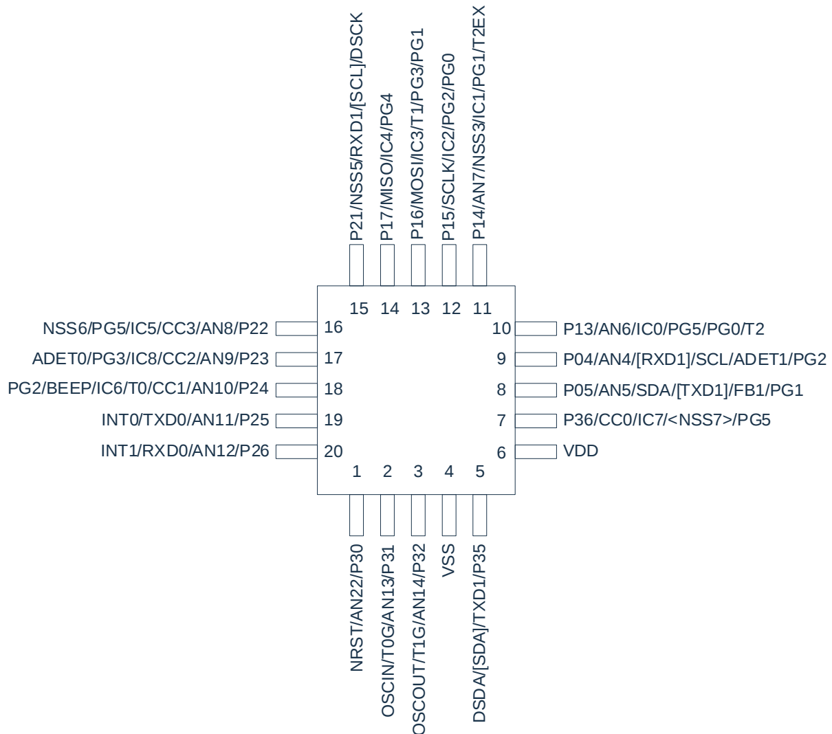
CMS8S5880-QFN20
