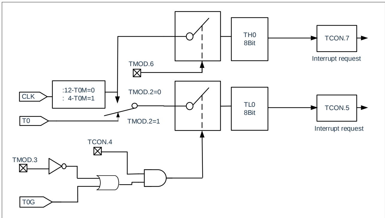
Figure 8-4: Timer0, Mode 3: Two 8-bit timer/counters
