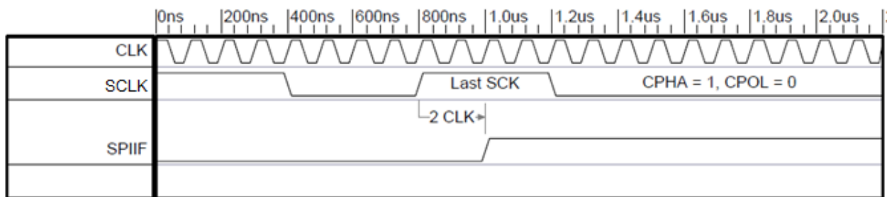
Figure 17-12: Interrupt generation
