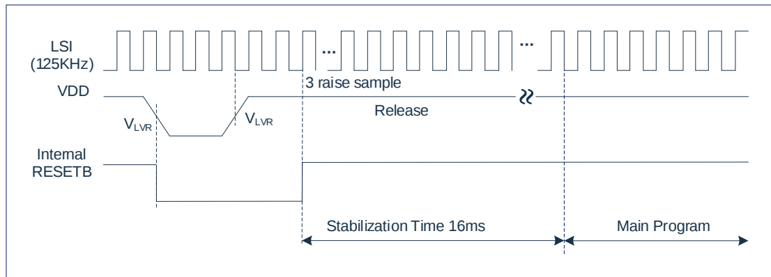
Figure 4-2:LVR Low Voltage Reset Timing Diagram
